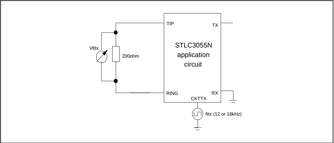
Figure 17. VTTX metering pulse level on line
